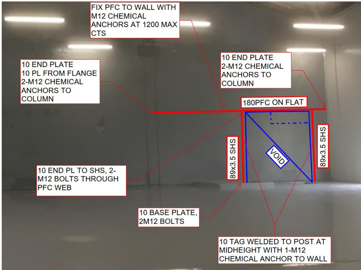
Panel Cut-out Strengthening Works
