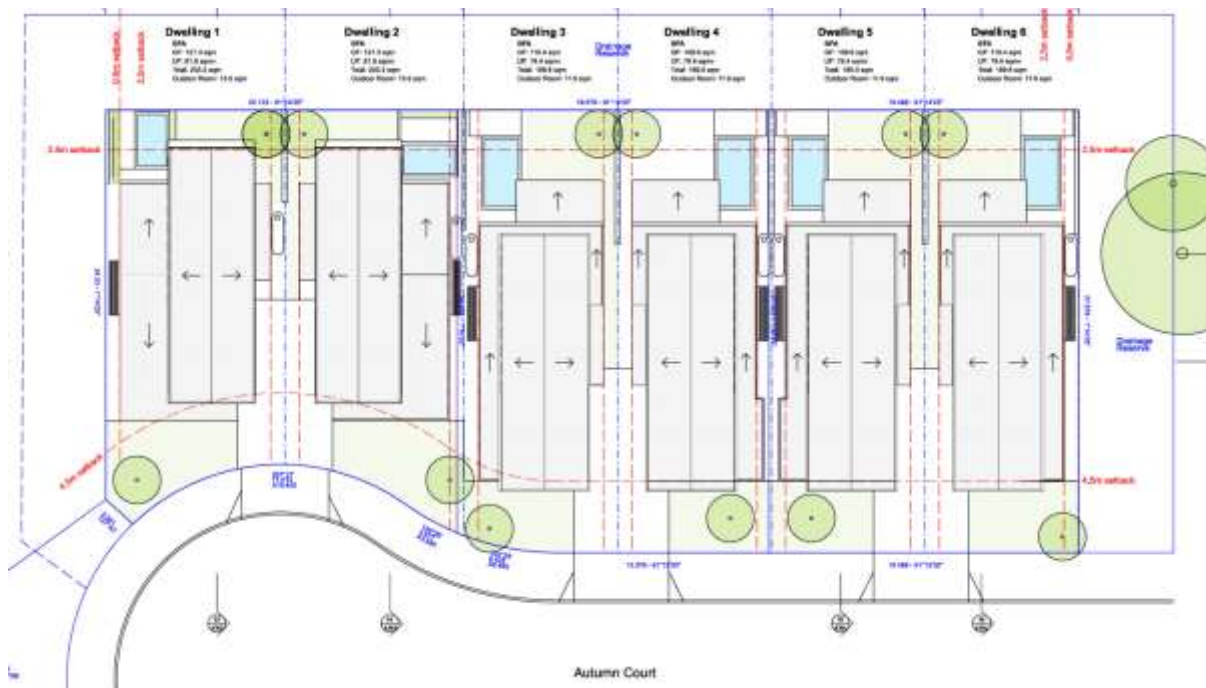
Figure 3: Site plan.
